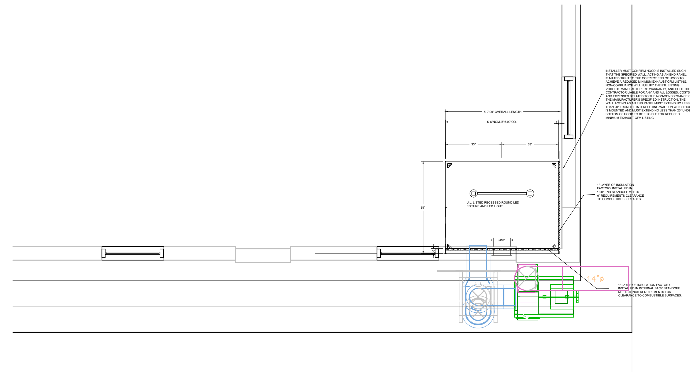
1 KITCHEN HOOD PLAN SK-1 3/8"=1'-0"
